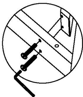
木牙螺钉安装示意图 Installation diagram of wooden tooth screws
