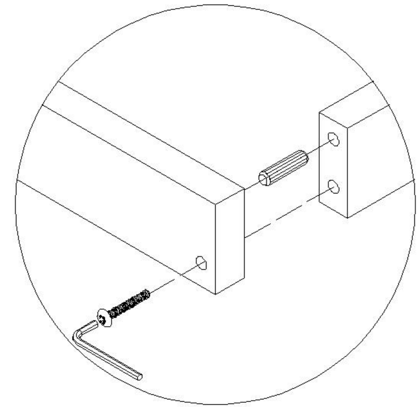
螺钉+木梢安装示意图 Installation diagram of screw + wooden tenon
