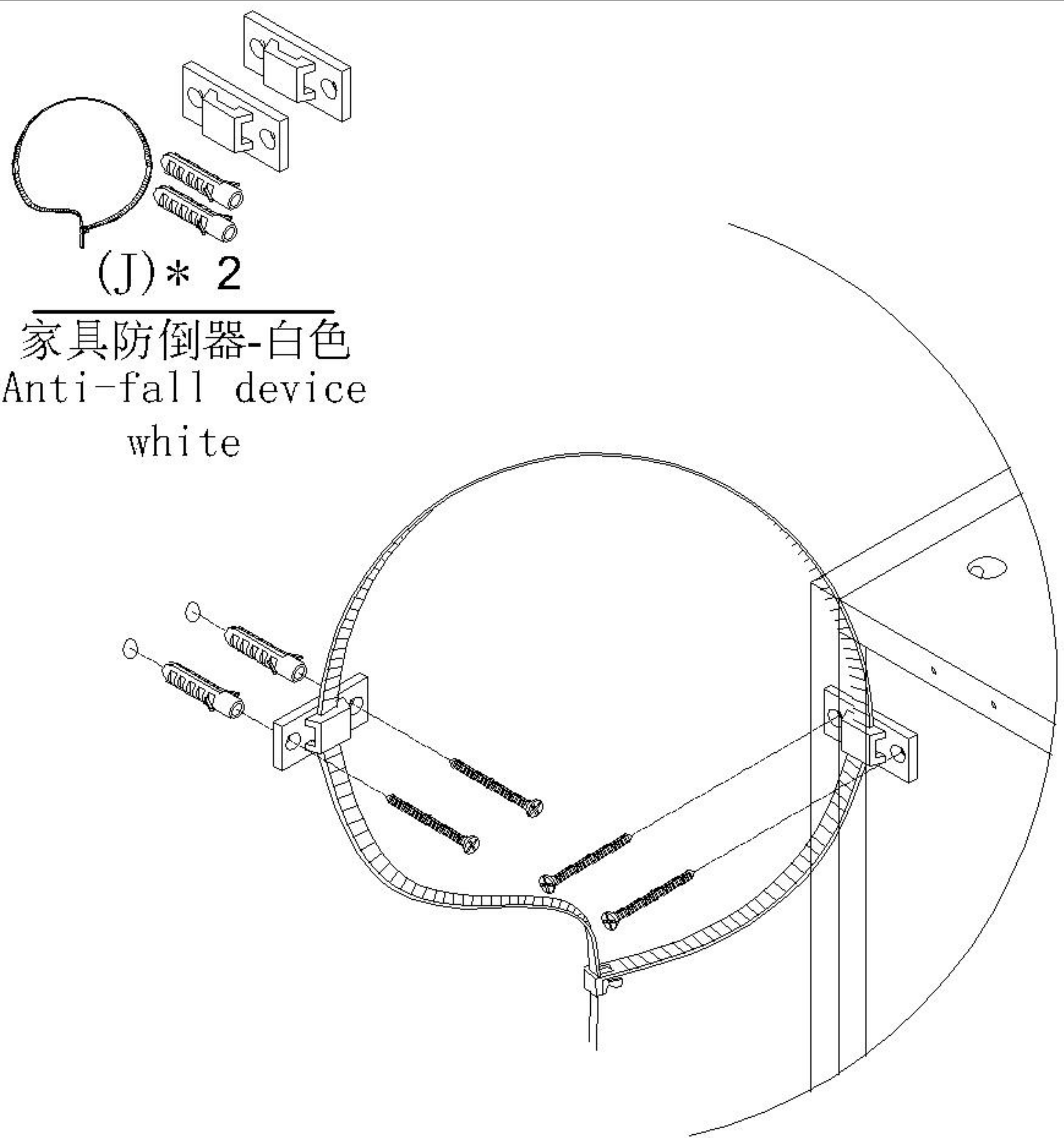
J处放大图 Enlarged view at J
