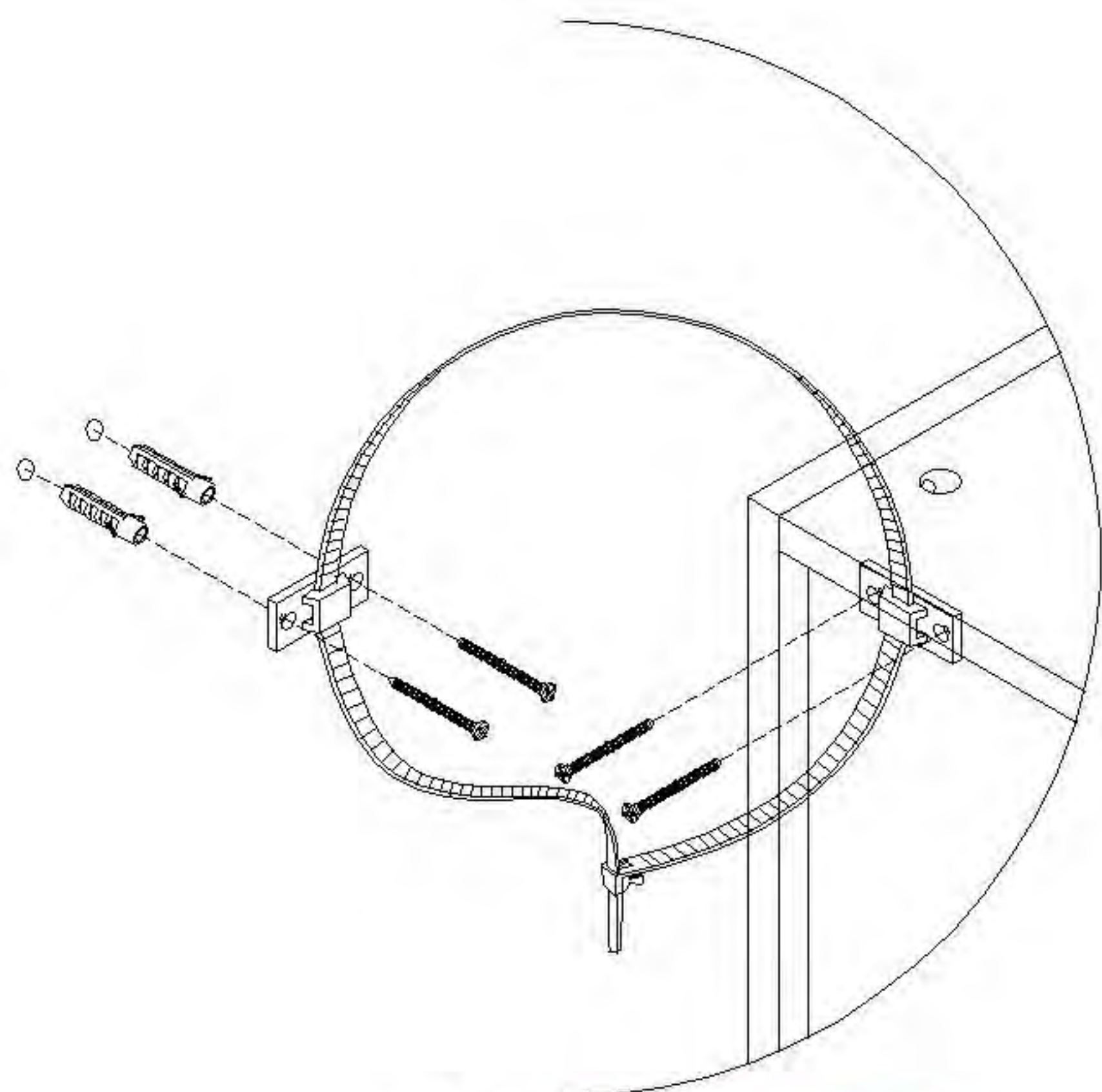
J处放大图 Enlarged view at J
