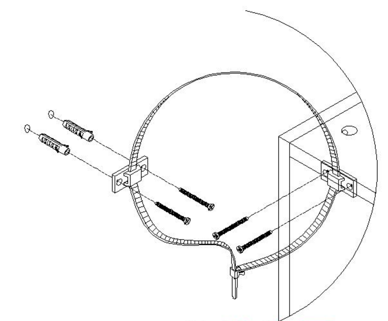
X处放大图 Enlarged view at X
