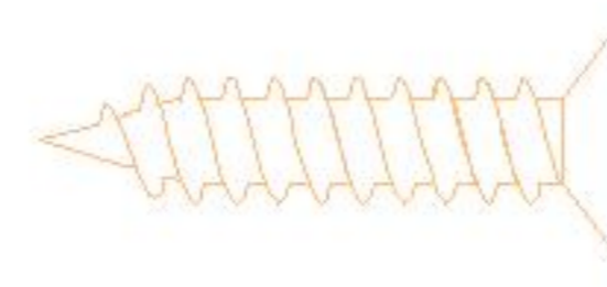
(J)*15 白攻螺丝M3.5*16mm Tapping screw
