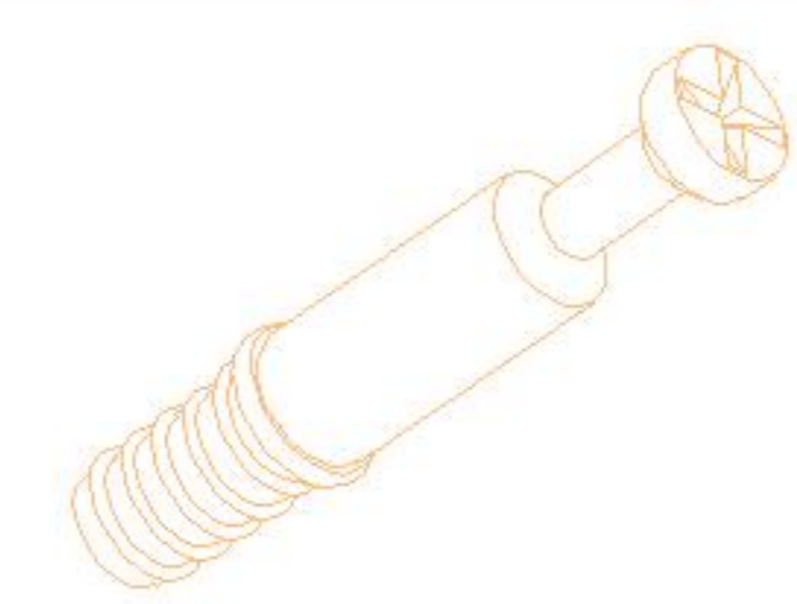
(A)*154 二合一螺杆 2-in-1-screw
