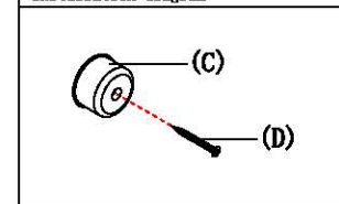
图3: 中脚安装示意图 Figure 3: Middle foot installation diagram
