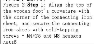
图2步骤1: 木脚弧度顶端对准连接铁片的角, 用自攻螺丝-M4*25和M8外六角螺母固定好连接铁片 Figure 2 Step 1: Align the top of the wooden foot's curvature with the corner of the connecting iron sheet, and secure the connecting iron sheet with self-tapping screws - M4*25 and M8 hexagon nuts
