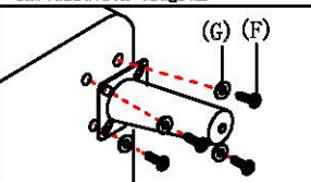
图3: 调节脚安装示意图 Figure 3: Schematic diagram of adjusting foot installation
