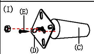
图1: 边脚安装示意图 Figure 1: Side foot installation diagram
