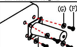
图3: 调节脚安装示意图 Figure 3: Schematic diagram of adjusting foot installation
