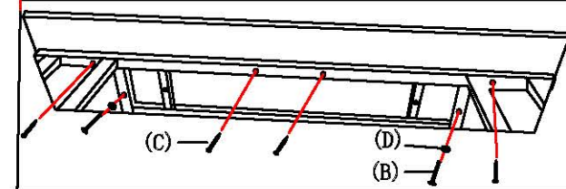
Installation diagram of the front panel of the seat frame
