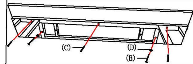
Installation diagram of the front seat panel
